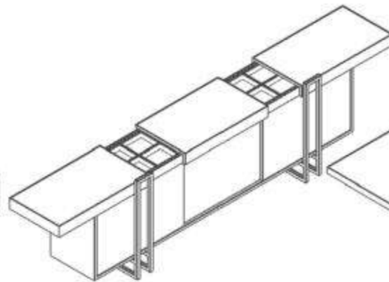
PLM.D 23641 L 236 W 41 H 85 cm
